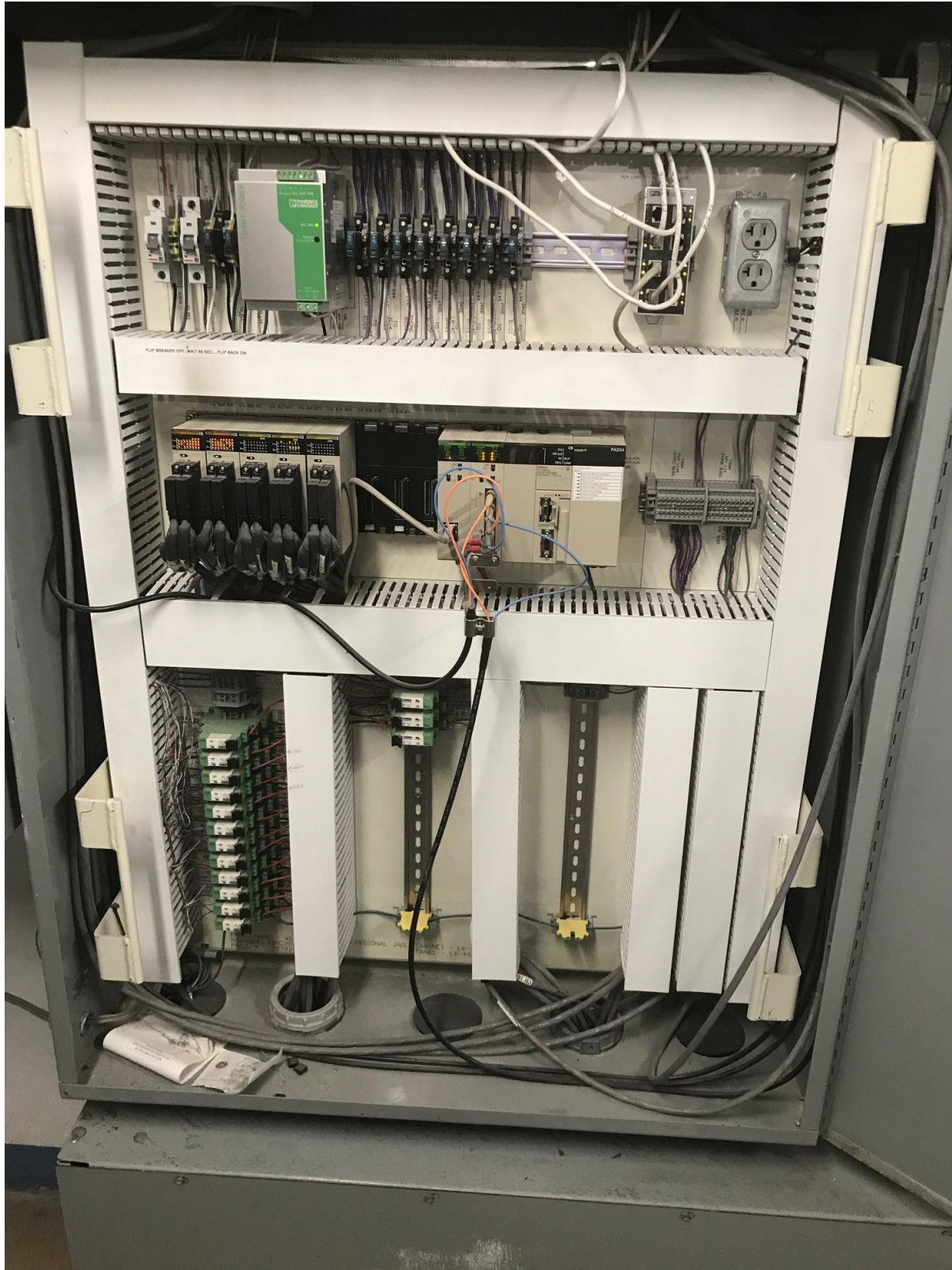
Pictured Below: PLC Cabinet 2
