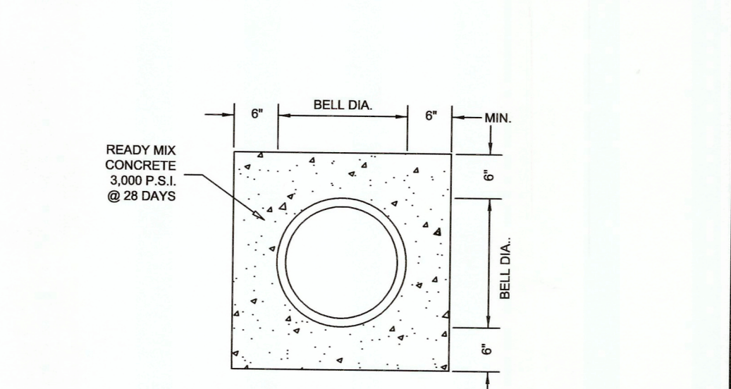
WESTERN VIRGINIA REGIONAL - CONSTRUCTION DETAIL CONCRETE ENCASED PIPE 01/01/14 G-9
