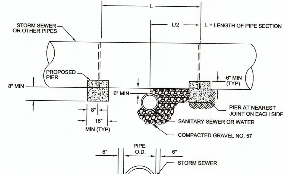
WESTERN VIRGINIA REGIONAL - CONSTRUCTION DETAIL CONCRETE PIER 01/01/14 G-8
