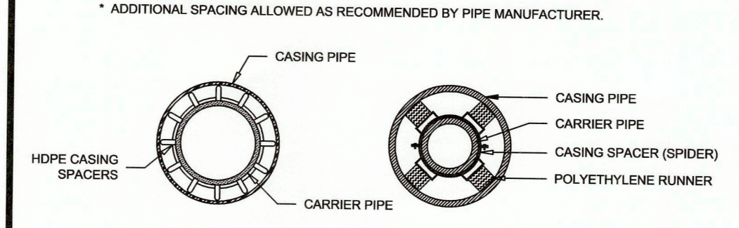
WESTERN VIRGINIA REGIONAL - CONSTRUCTION DETAIL PIPE SUPPORT IN CASING PIPE 05/01/15 G-6
