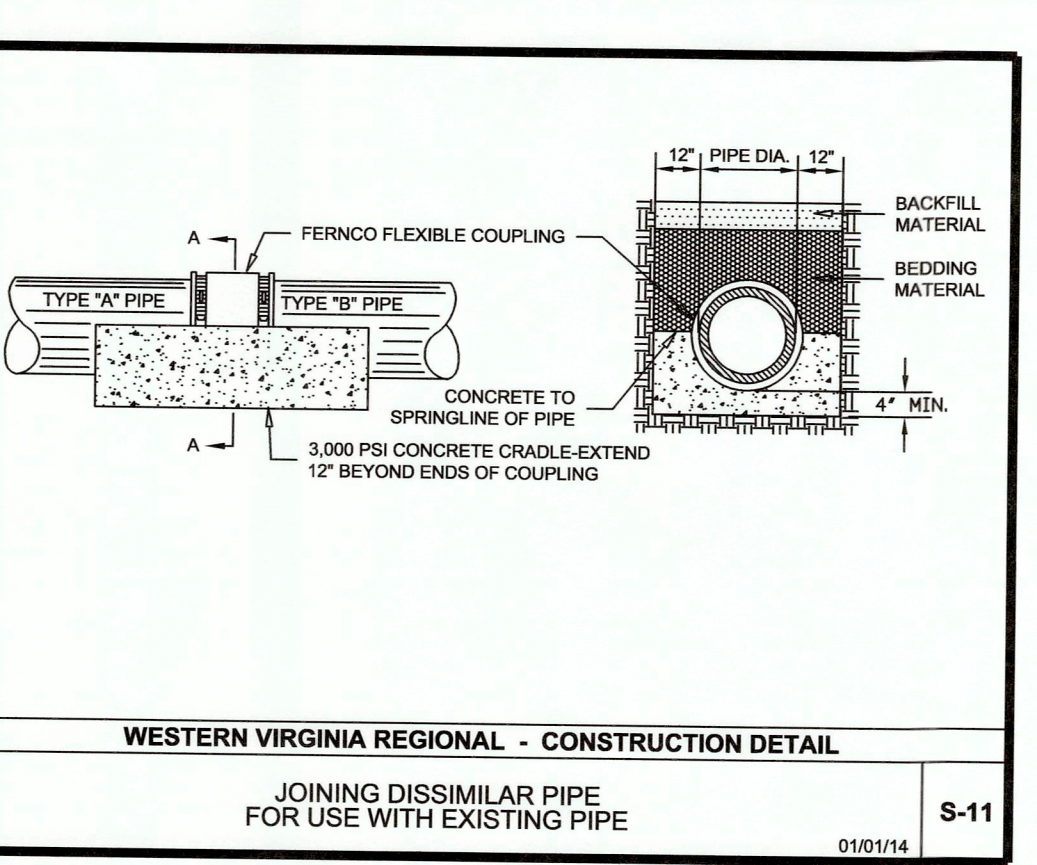
WESTERN VIRGINIA REGIONAL - CONSTRUCTION DETAIL JOINING DISSIMILAR PIPE FOR USE WITH EXISTING PIPE 01/01/14 S-11
