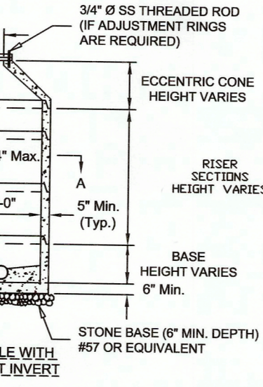
WESTERN VIRGINIA REGIONAL - CONSTRUCTION DETAIL 4" STANDARD MANHOLE FOR PIPE 15" OR SMALLER (FOR DEPTHS UP TO 15 FEET) 08/01/15 S-1
