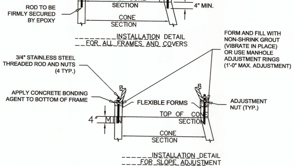
WESTERN VIRGINIA REGIONAL - CONSTRUCTION DETAIL WATERTIGHT MANHOLE FRAME 01/01/14 S-4
