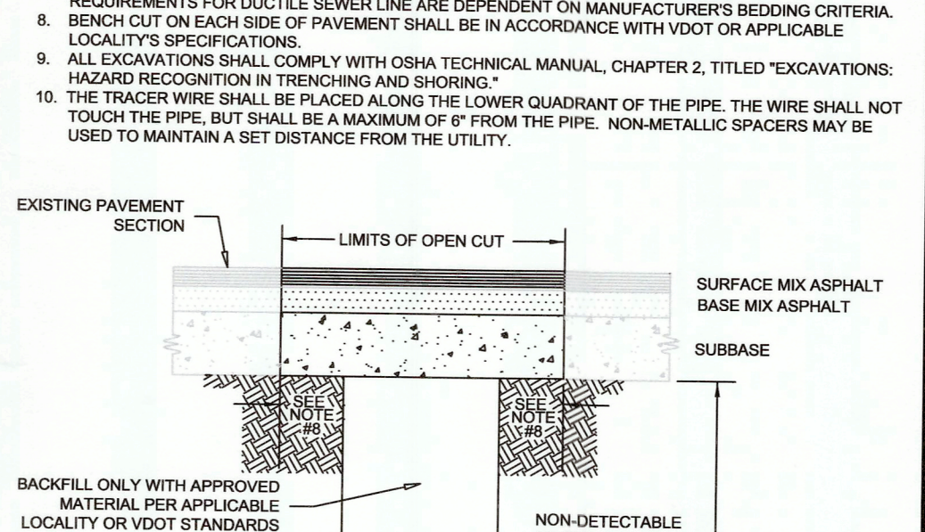
WESTERN VIRGINIA REGIONAL - CONSTRUCTION DETAIL BEDDING AND BACKFILL UNDER PAVEMENT AND IN RIGHT-OF-WAY 08/01/15 G-12
