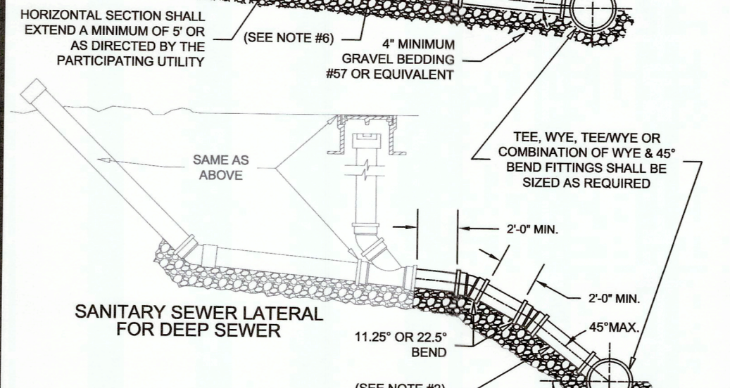
WESTERN VIRGINIA REGIONAL - CONSTRUCTION DETAIL SANITARY SEWER LATERAL 01/01/14 S-6
