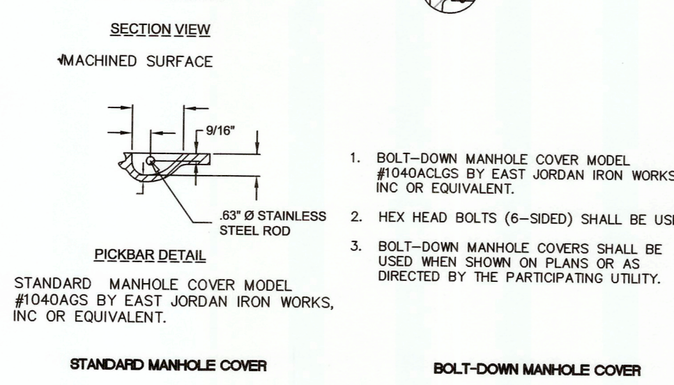
WESTERN VIRGINIA REGIONAL - CONSTRUCTION DETAIL WATERTIGHT MANHOLE COVER 01/01/14 S-5
