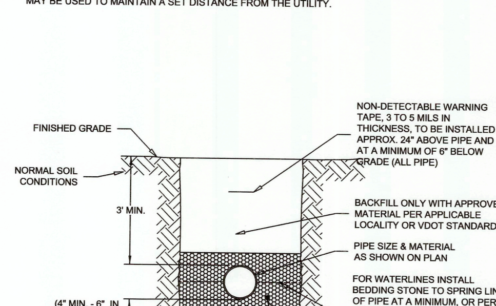
WESTERN VIRGINIA REGIONAL - CONSTRUCTION DETAIL BEDDING AND BACKFILL OUTSIDE OF PAVED AREAS 08/01/15 G-11
