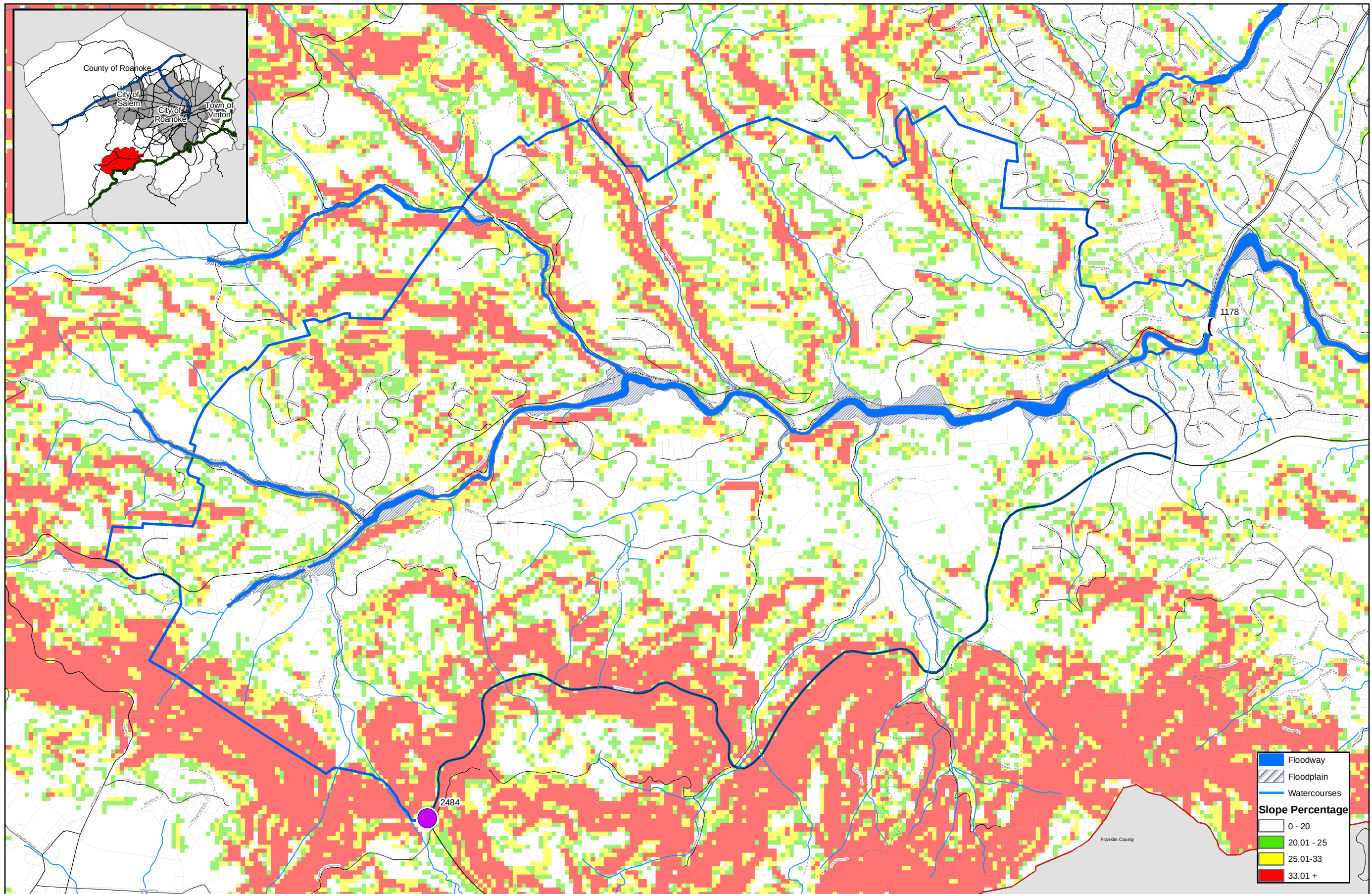
Map 2.14 Route 221 Area Plan: Slope
