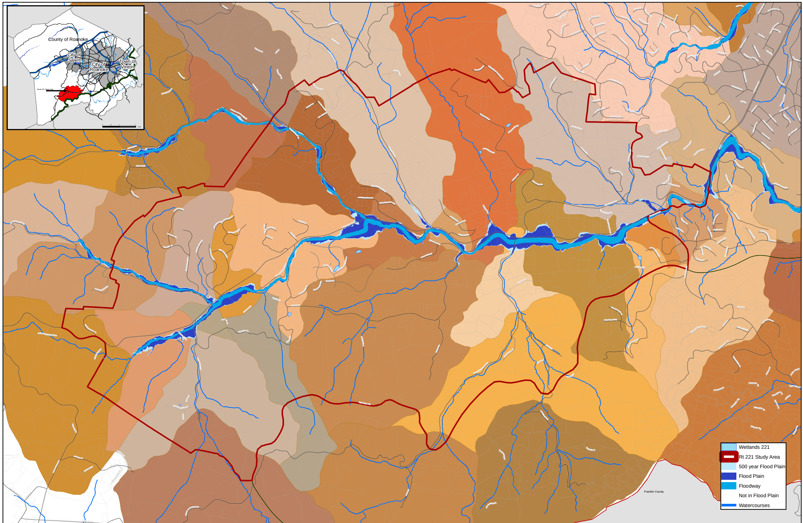
Map 2.11 Route 221 Area Plan: Drainage Areas
