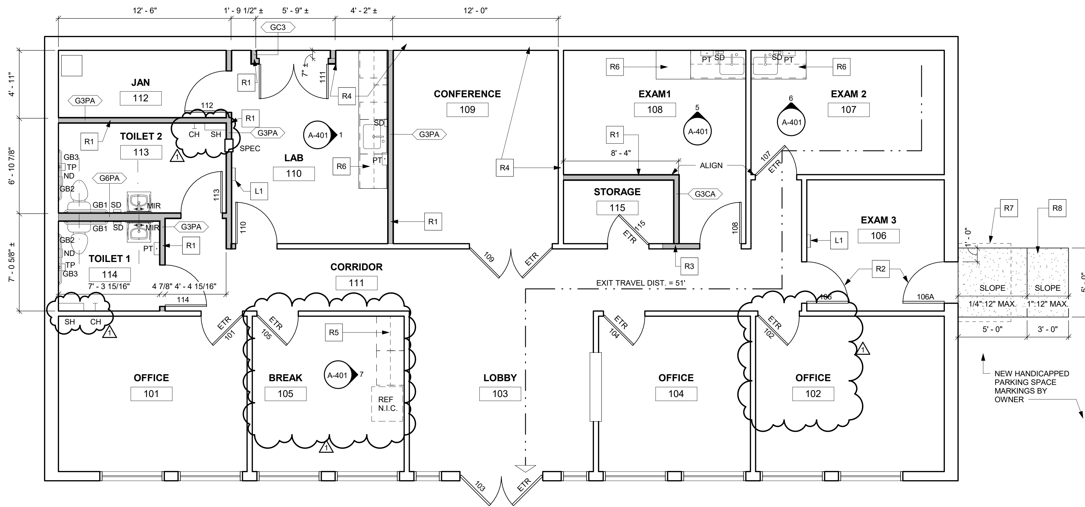
1 A-101 1/4" = 1'-0" FIRST FLOOR PLAN
