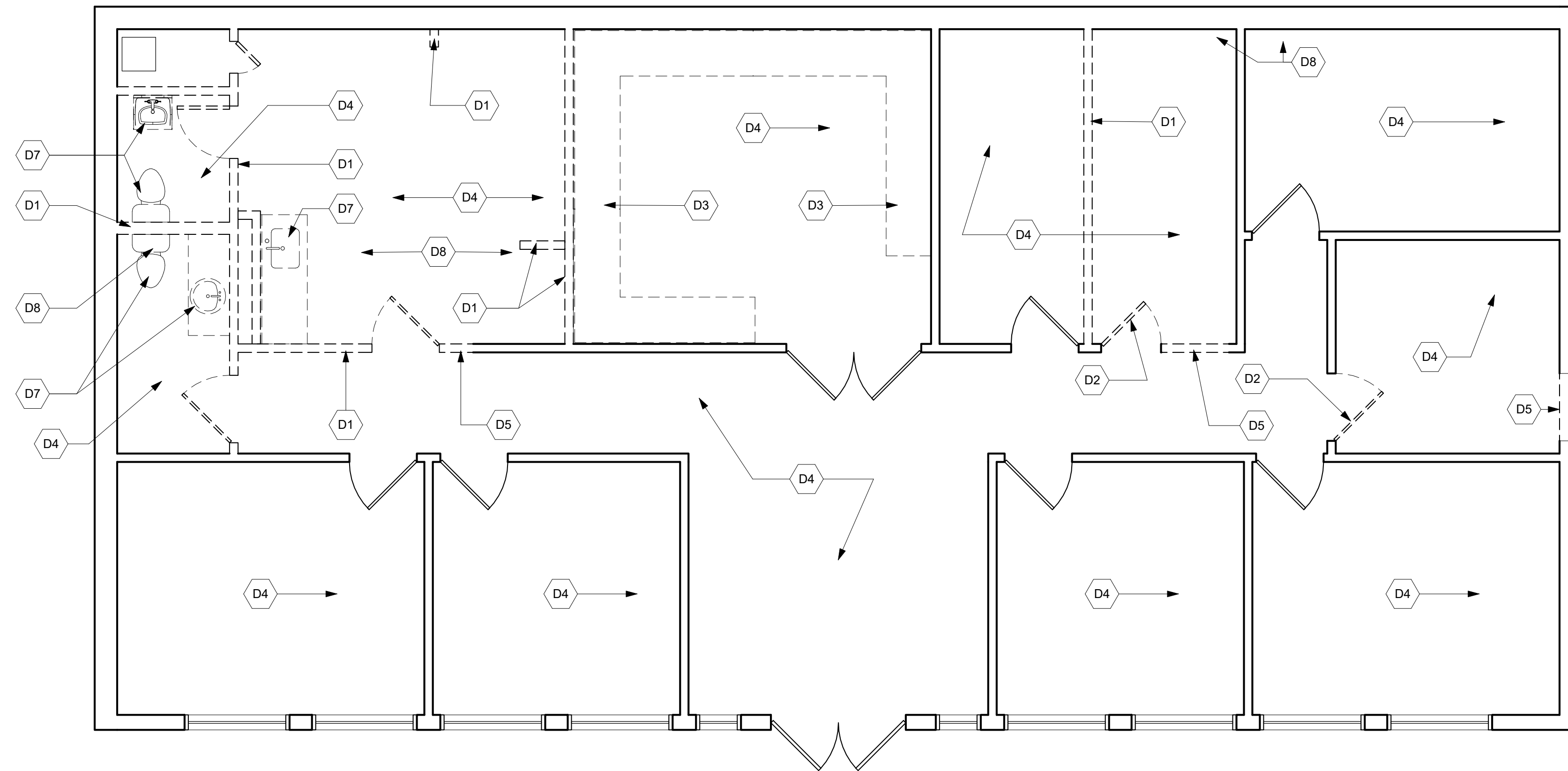
2 A-101 1/4" = 1'-0" DEMOLITION PLAN
