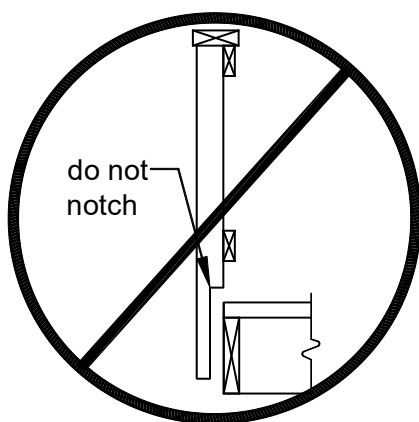
FIGURE 36: POST NOTCHES PROHIBITED PER GUIDE
